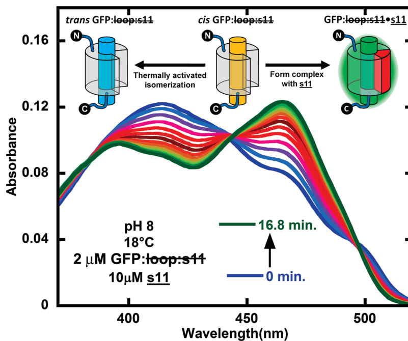
Figure 3. Competition between cis \rightarrow trans thermal isomerization and binding of s11 to cis -GFP: \beta 23-48 to form GFP: \beta 23-48 \cdot s11 starting from the initial photostationary mixture of refolded GFP: \beta 23-48 generated by light-activating trans -GFP: \beta 23-48 with 460 nm light (blue). The spectra following from blue to green are shown for every 1.2 min after mixing in s11 in the dark. The cartoon inset shows the kinetic model that describes the processes taking place, namely cis -GFP: \beta 23-48 is partitioning between binding s11 to form GFP: \beta 23-48 \cdot s11 and reverting back to trans -GFP: \beta 23-48. The initial concentrations of trans -GFP: \beta 23-48 and s11 were 2 \mu M and 10 \mu M , respectively, and they were in pH 8 buffer at 18^\circ C .
