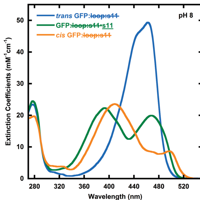
Figure 4. Absorbance spectra of cis -GFP: \beta 23-48 (yellow), trans -GFP: \beta 23-48 (blue), and GFP: \beta 23-48 \cdot s11 (green). The absorbance spectra of GFP: \beta 23-48 \cdot s11 (green) and trans -GFP: \beta 23-48 (blue) are reproduced from Figure 1B for comparison. The cis -GFP: \beta 23-48 absorbance spectrum is derived from observing the changes in the photostationary state of GFP: \beta 23-48 with pH and photoactivation wavelength. These absorbance spectra are used to fit the data in Figures 2 and 3 to determine the concentrations of cis -GFP: \beta 23-48, trans -GFP: \beta 23-48, and GFP: \beta 23-48 \cdot s11 .
